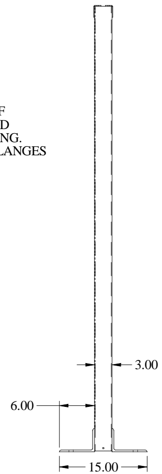
SIDE VIEW
